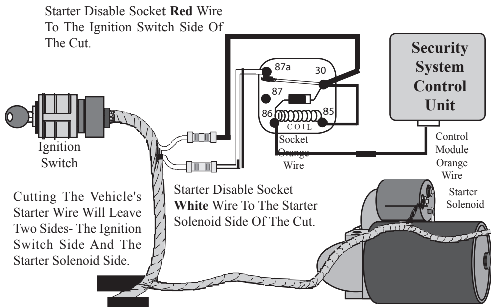
Configuring A Starter Disable Using The AU-SOCKET And SPDT Relay.
