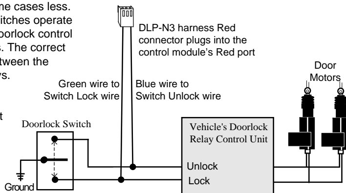
3 Wire Negative Doorlocks using the AL-100-H Control Unit outputs
