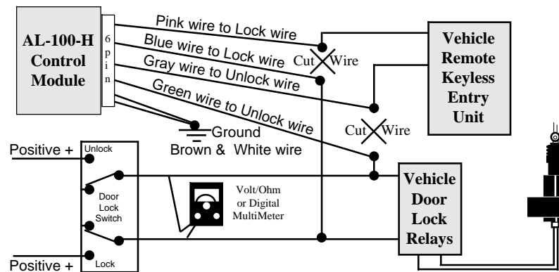
Type 1 Connection: Meter shows polarity change before the Lock and Unlock wires are cut. The doorlock relays and RKE unit are also separate.
