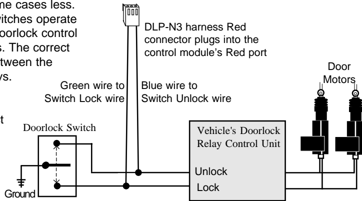
3 Wire Negative Doorlocks using the AL-100F Control Unit outputs
